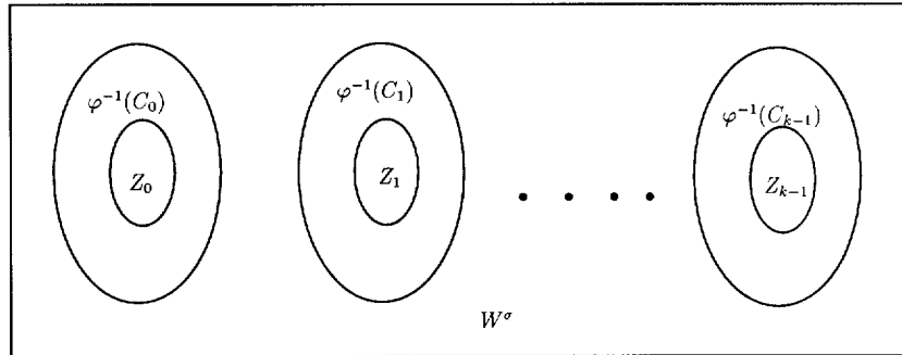
Fig. 6. For all 0 \leq t < k , \varphi^{-1}(C_t) consists of vertices coloured by the colours from C_t . The sets \varphi^{-1}(C_t) are pairwise disjoint, each of them contains a subset Z_t , where player \sigma has a memoryless winning strategy z_t^\sigma . If the token is in \varphi^{-1}(C_t) \setminus Z_t = \text{Attr}^\sigma(G[W^\sigma], N_t) \setminus N_t , then player \sigma can use the attracting strategy \text{attr}^\sigma(G[W^\sigma], N_t) to force the token outside of \varphi^{-1}(C_t) , i.e. to N_t = W^\sigma \setminus \varphi^{-1}(C_t) .
