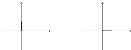
FIGURE 3. The segment (0, a^*) (left) and the segment (0, b^*) (right).
