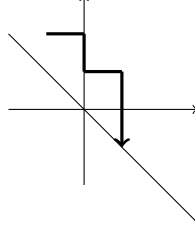
FIGURE 4. An example of a finite dual strand coded by the word babaa . The arrow at the end of the path indicates that we read the letters from left to right.
