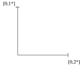
FIGURE 2. The segments \overline{[0, 1^*]} and \overline{[0, 2^*]} .
