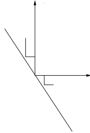
FIGURE 3. A piece of the stepped surface for 1 \mapsto 121 , 2 \mapsto 12 .
