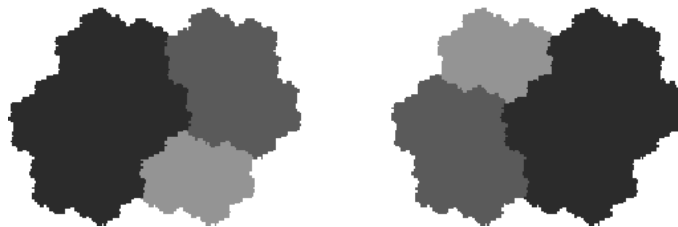
Figure 10.3. The exchange map E .
