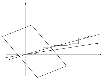
Figure 10.1. The Rauzy broken line.
