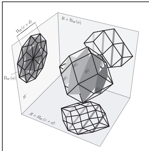
Figure 1: Window for the Penrose tiling.
