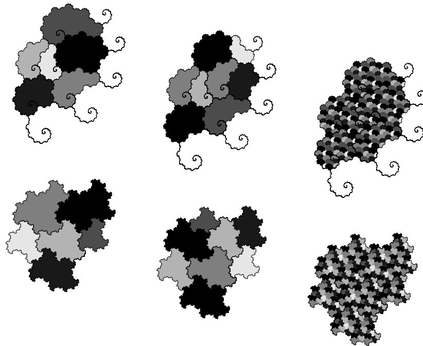
Figure 4: Nautilus and Conch tiles, and substitution. These shapes form windows for the substitution tilings generated by the rule in Figure 3.
