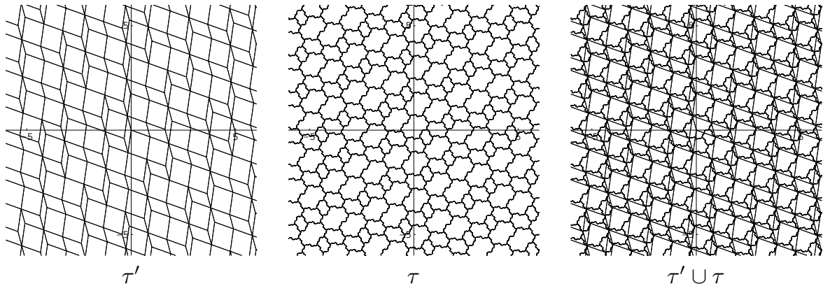
Figure 4: \tau' , \tau , and \tau' \cup \tau on Example.
