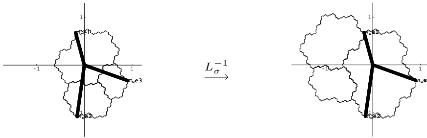
Figure 3: \{X_i\}_{i=1,2,3} and \{L_\sigma^{-1} X_i\}_{i=1,2,3} on Example.
