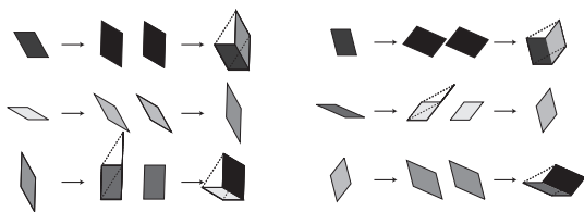
Figure 3: The substitutions generated by the morphisms \sigma_1 and \sigma_2 on their boundaries
