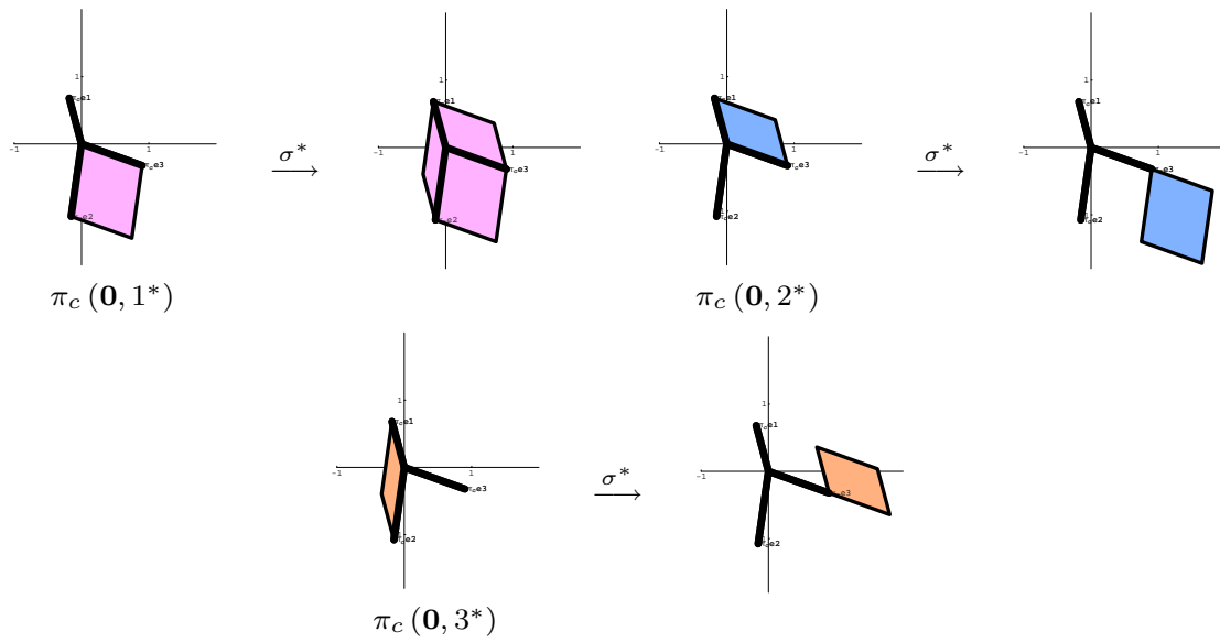
Figure 1: The tiling substitution \sigma^* on Example.
